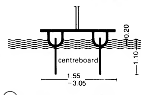
21 Open catamaran: section
